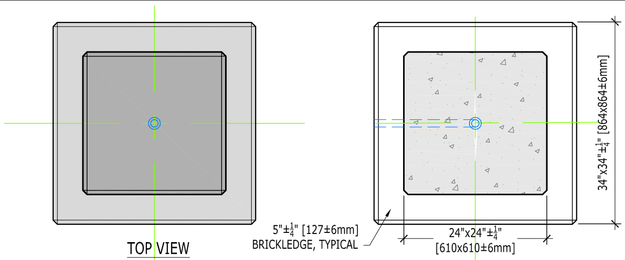
HORIZONTAL SECTION
