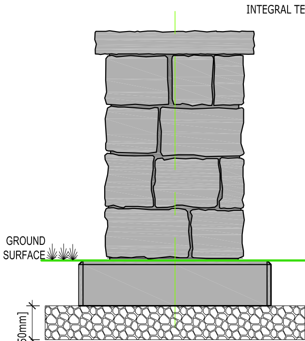
SIDE VIEW - INSTALLATION
