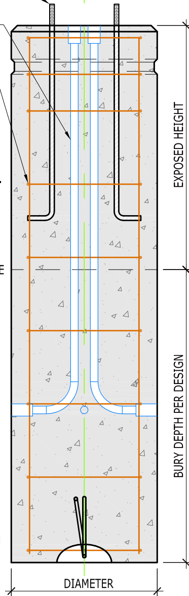
VERTICAL SECTION
